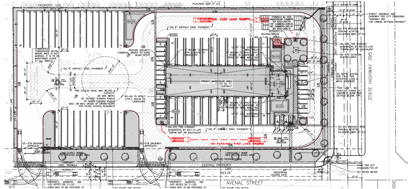
Figure 3 - Draft Site Plan
