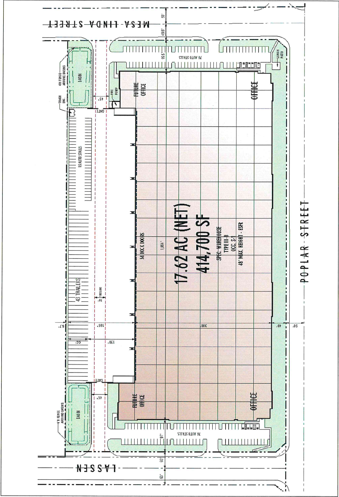
FIGURE 2 Site Plan Poplar 18 Project
